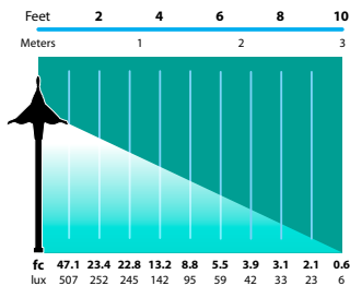
AL-14 Half Spread Photometrics 20 ft. (6.1m) diameter
