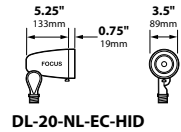
DL-20-NL-EC-HID
