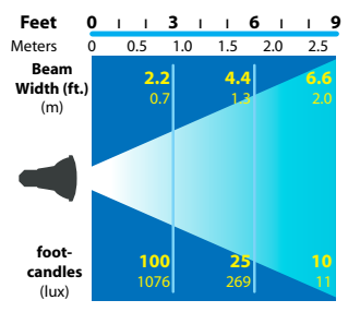
50w PAR20 Flood 40°
