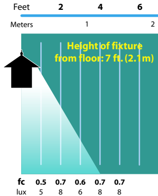
SL-12 Half Spread Photometrics 8 ft. (2.4m) diameter
